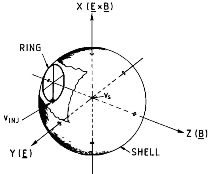
Figure 6.2: Ring and shell distributions of pickup ions arising from the interaction of a cometary exosphere with the solar wind Coates et al. (1990).
