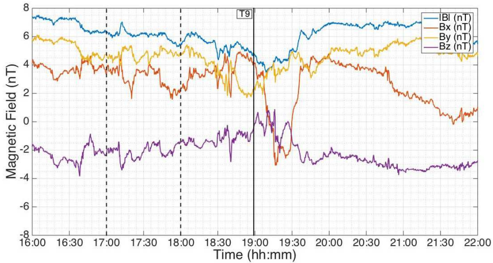
Figure 5.14: Magnetic field data in TIS coordinates three hours before and after closest approach. The dashed vertical lines indicate the boundaries of the time period from which the MIMI/CHEMS spectra shown in Figure 5.13 were obtained.
