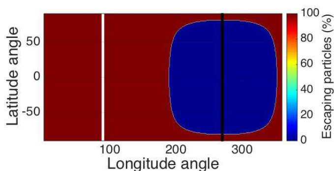
Figure A.1: Equirectangular projection of Titan's exobase showing the percentage of 1 keV electrons that are able to escape the moon's vicinity during a backward tracing under a uniform background magnetic field. The white vertical line indicates the position of the ram direction while the black vertical line indicates the position of the tail.
