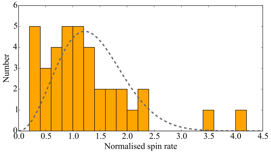
Figure 6.1: Histogram of the normalised rotation rates of 37 JFCs. The normalised spin rate is calculated as f/\langle f \rangle where f = 1 / P_{\text{rot}} and \langle f \rangle is the geometric mean of f . The dashed line corresponds to the best-fitting Maxwellian distribution.
