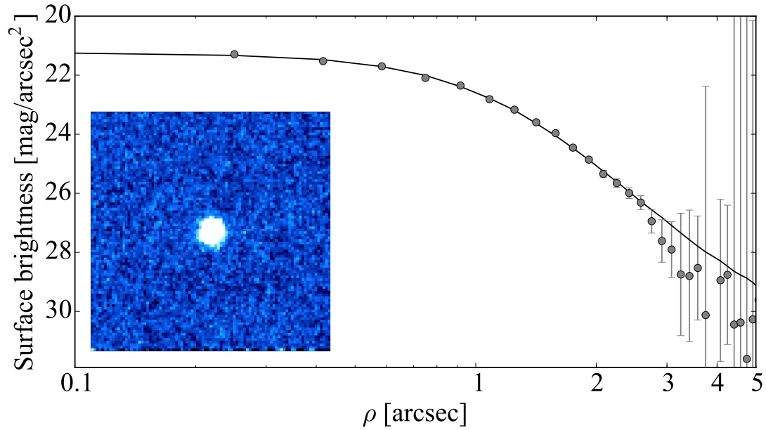
Figure 7.17: Same as Fig. 7.1, for the observations of 162P from 18 February 2017. The composite image in the lower left corner was made up of 9 \times 120 s exposures.
