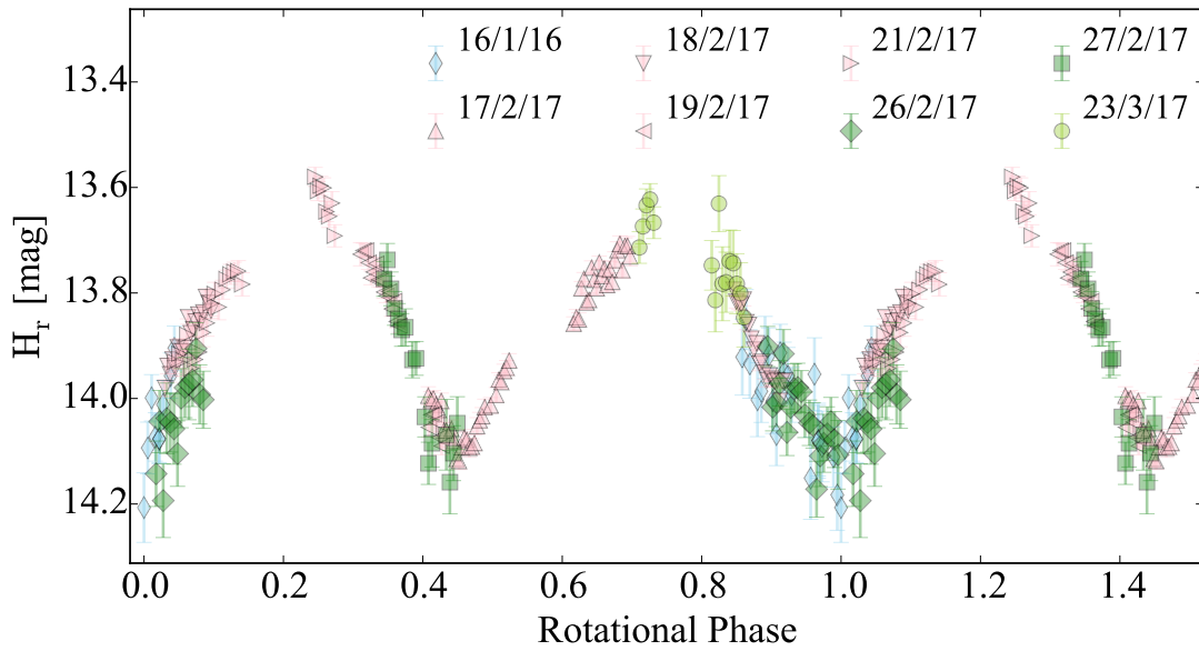
Figure 7.13: Rotational lightcurve of comet 143P from the data taken in 2016 and 2017. The magnitudes from 17-21 February and from 26-27 February were derived using the same set of comparison stars and are therefore plotted in the same colours. This lightcurve was corrected for a phase-function slope \beta = 0.051 mag/deg and was phased with a period P = 17.1966 h. It corresponds to the best lightcurve from the MC2 test.
