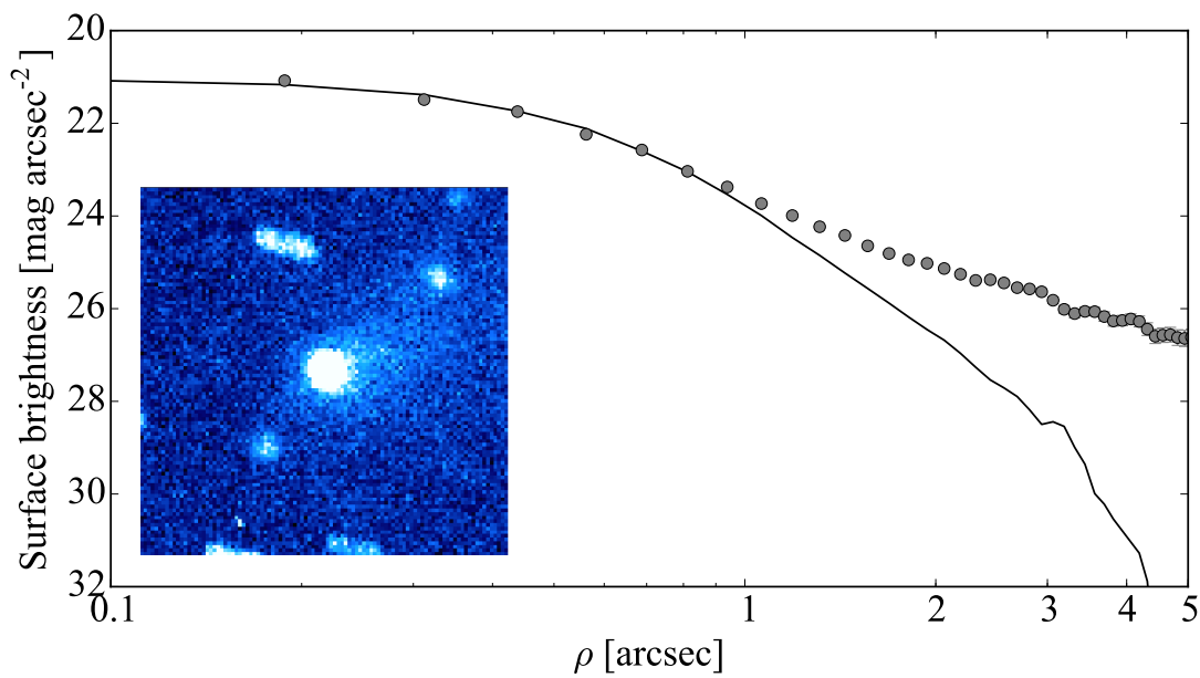
Figure 5.20: Same as Fig. 5.1, for the VLT observations of 93P on 24 January 2009. Due to the small number of frames, the composite image was made without subtraction of the average stellar background in order to avoid artefacts from the comet’s slow position change. The co-added composite image is made up of 8 \times 250 s exposures. A tail to the west can be clearly distinguished. The comet profile appears stellar close to the centre but deviates from that of the comparison star at larger radii.
