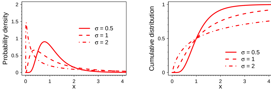
Figure 3.9: Log-normal probability density functions (left panel) and cumulative distribution function functions (right panel) with location parameter \mu = 0 and various values of \sigma (see legend inset).
