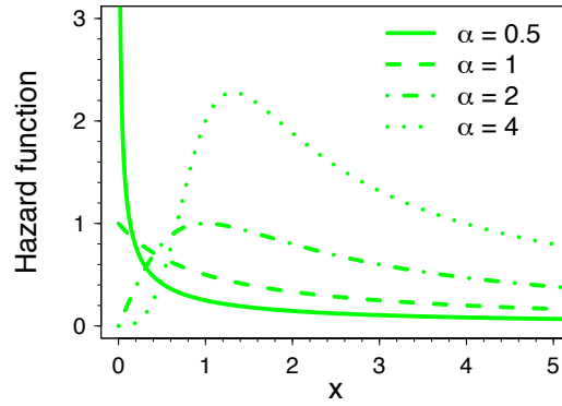
Figure 3.12: Hazard functions of the log-logistic distribution (3.56) for a scale parameter \theta = 1 and various values of the shape parameter \alpha as given in the legend.
