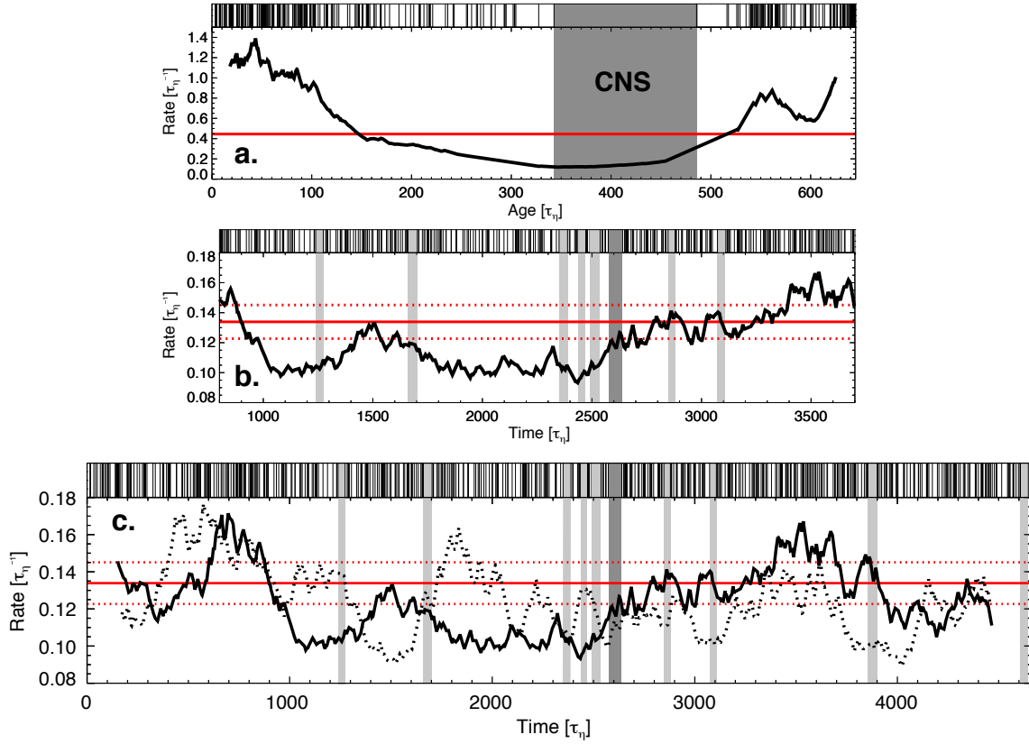
Figure 6.1: Panel a : Geomagnetic reversal rate during the past 158 Myr from the polarity time scale of Ogg (2012). Time has been rescaled using the outer core magnetic diffusion time \tau_\eta = 244 kyr based on the electrical conductivity estimates of Pozzo et al. (2012). The Cretaceous normal superchron (CNS) is highlighted in gray. The horizontal line shows the mean reversal rate. Panels b and c : Reversal rate throughout the simulation run of model M2 for a period containing roughly the same number of reversals as the paleomagnetic record (panel b) and for the complete run (panel c). The solid horizontal line represents the estimated rate from the exponential distribution fit of the stable polarity intervals obtained using the threshold combination \mathcal{M}_C = 0.3 , \mathcal{T}_S = 0.2 . Dotted lines mark the 95% confidence interval of the rate estimate. The dotted curve in panel c shows the reversal rate for a synthetic data set obtained drawing random samples from an exponential distribution with the above rate. Colored backgrounds highlight the longest polarity interval (dark gray) and polarity intervals longer than 30 \tau_\eta (light gray). All the reversal rate estimates have been calculated using a sliding window with a fixed number of N = 40 reversals.
