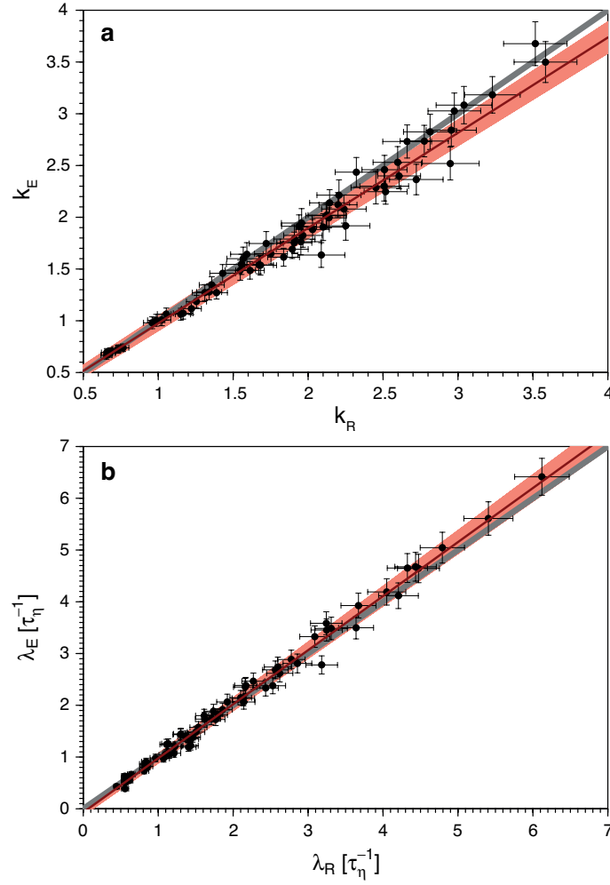
Figure 5.35: Estimated gamma distribution parameters (shape k in panel a and rate \lambda in panel b) for reversal durations (subscript R ) and grand excursion durations (subscript E ). Each plotted symbol refers to a combination of \mathcal{M}_C and \mathcal{T}_S explored. Error bars represent the 68% confidence intervals of the relative estimate. The grey background line in panel a (panel b) indicates k_E = k_R ( \lambda_E = \lambda_R ). Linear least-squares fits are shown in red with the color shaded backgrounds representing the respective 95% confidence intervals.
