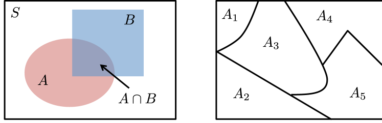
Figure 3.1: Left panel : Relationship between the sample space S and the sets A and B in the definition of conditional probability. Right panel : Decomposition of the sample space S into the disjoint sets A_i , i = 1, \dots, 5 .
