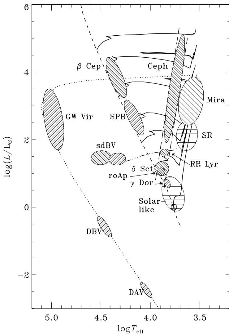
Figure 7. Hertzsprung-Russell diagram showing the location of the principal types of asteroseismic variable stars discussed below.
