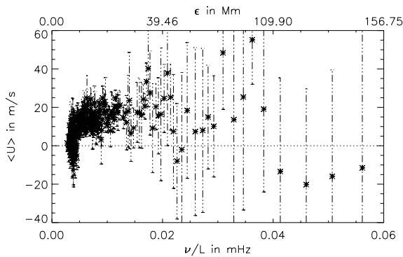
Fig. 2 Estimated integrated horizontal meridional velocity on the northern hemisphere of the Sun as a function of \nu/L and mode penetration depth \epsilon .
