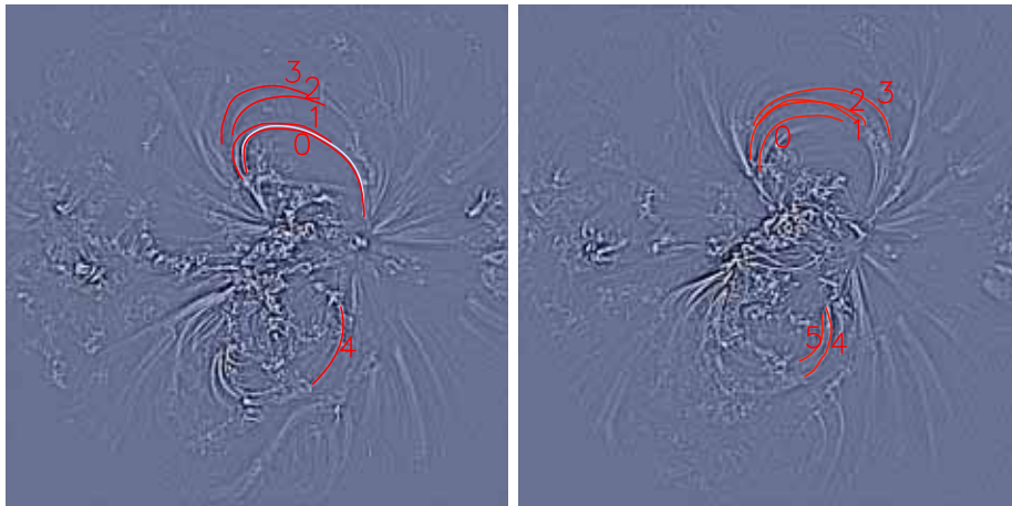
Figure 4. Hand-traced loops (red lines) marked with numbers on the filtered TRACE 171 Å images observed on 1 March, 1422UT (left) and 2 March, 1744UT (right). In the left image, the white line is segmented out from another TRACE image which is observed on 1 March, 1351UT and then transformed its coordinate onto 1 March, 1422UT.
