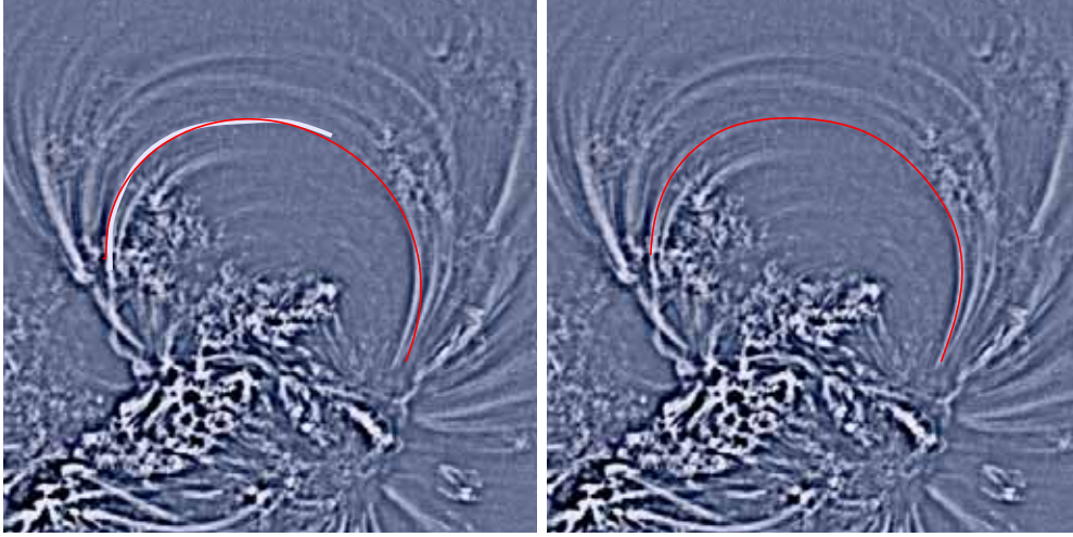
Figure 10. Left: the white line shows the traced partial Loop 0 in Image B and the red line is the best fitting field line b(0,0) with this loop. Right: the red line shows the extended complete loop with the guide of the field line b(0,0) .
