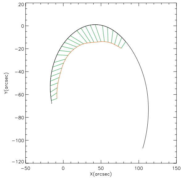
Figure 7. This figure illustrates how the parameter C_L(b) is calculated. Red line is one traced loop, black line is one projected magnetic field line and Green sticks show the area between the loop and the part of the field line corresponding to the loop.
