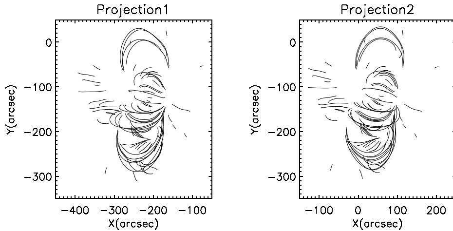
Figure 6. Projection results of the extrapolated 3D potential field lines along two TRACE view directions. The left image is for the viewpoint on 1 March, 1422UT and the right one on 2 March, 1744UT.
