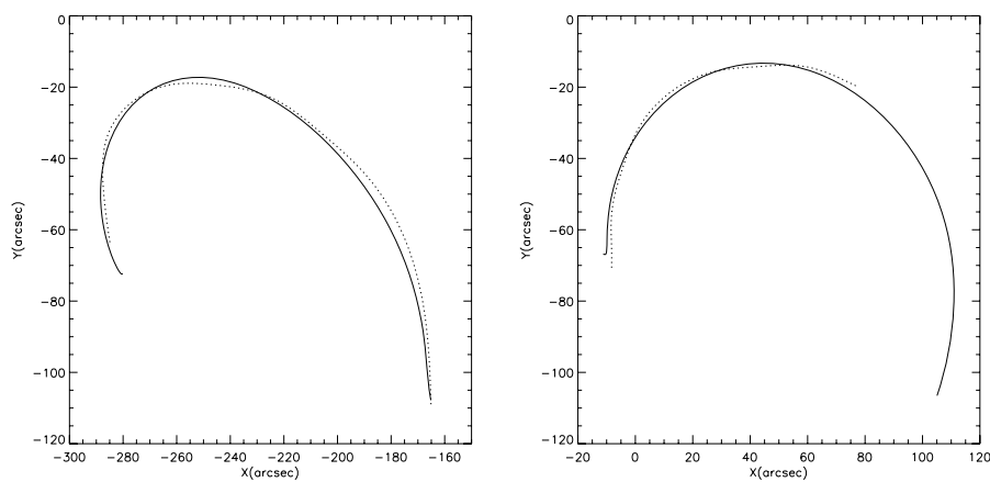
Figure 9. Dotted lines: loop No.0 in Image A (left) and loop No.0 in Image B (right); Solid lines: projections of the best fitting field line onto the respective image, we use b(0,0) as the notation for this field line.
