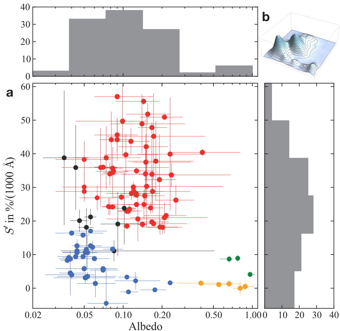
Fig. 2.— a) Color-albedo diagram for 109 TNOs showing two main clusters, one composed of Dark Neutral objects (blue points, albedos \sim 0.05 and S' \sim 10\% ), and another of Bright Red objects (red points, albedo \sim 0.15 and S' \sim 30\% ). Black points have large uncertainties and ambiguous surface type. Large TNOs (green) and objects with Haumea-type surfaces (orange) occupy a third group (bottom right corner). Albedo and color histograms are shown in grey. b) Smooth 2D histogram (Gaussian kernel with width 3% of full ranges, weighted by error bars) of the color-albedo distribution shown in a).
