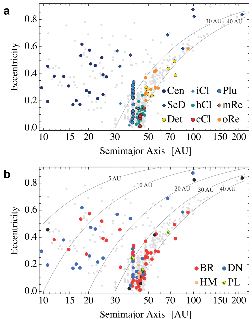
Fig. 1.— a) Orbital distribution (semimajor axis vs. eccentricity) of our sample (Cen=Centaur, iCl=Inner Classical, Plu=Plutino, ScD=Scattered Disc, hCl=Hot Classical, mRe=Middle Resonant, Det=Detached, cCl=Cold Classical, oRe=Outer Resonant). Light gray points mark TNOs not observed by Herschel. Curves of constant perihelion are plotted in solid gray and labelled. b) Same as a) but color-coded by surface type (BR=Bright Red, DN=Dark Neutral, HM=Haumea-type, PL=Dwarf Planets, black points have large uncertainties and ambiguous surface type.)
