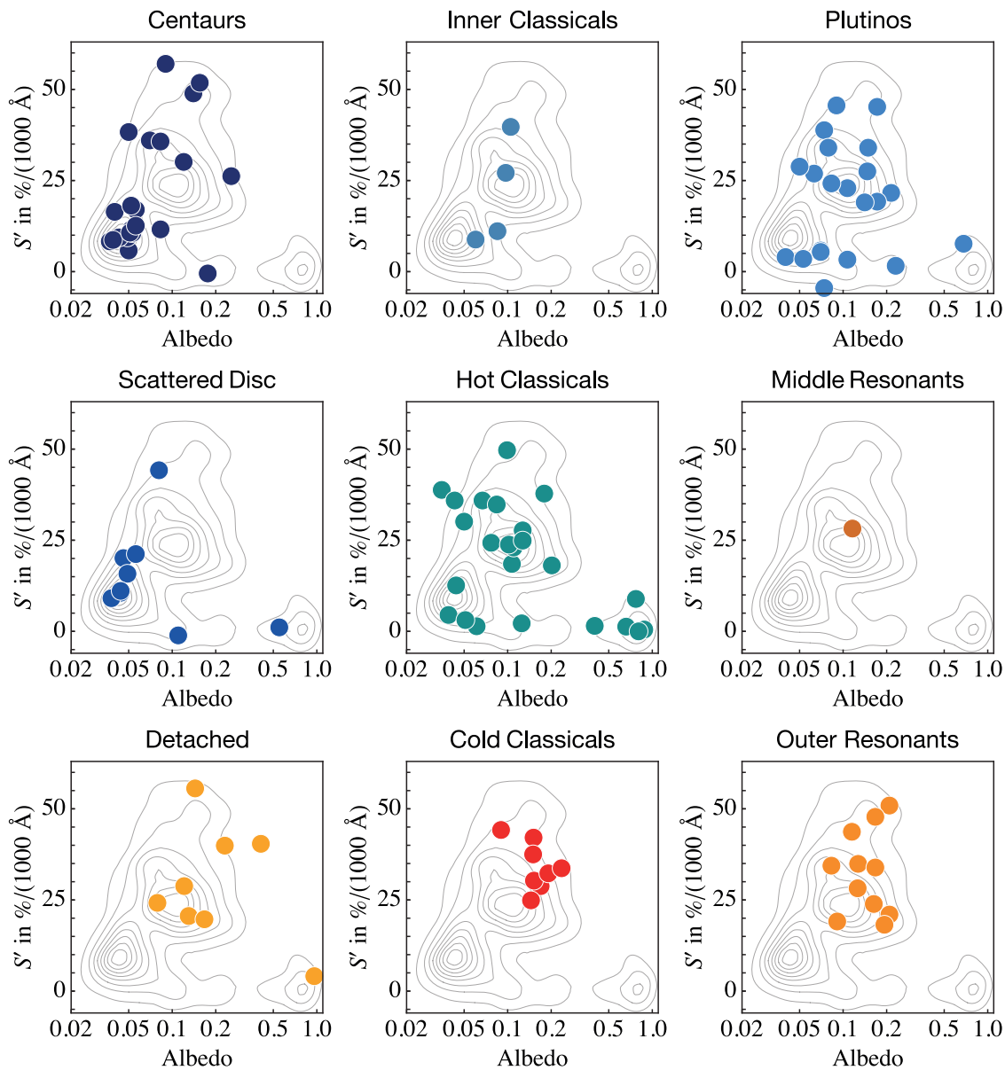
Fig. 3.— Same as Figure 1 with objects gathered by dynamical class. Underlying contours are a density map of all objects obtained by bootstrap-sampling each object 100 times assuming its albedo (color) follows a lognormal (normal) distribution set by the observing uncertainties.
