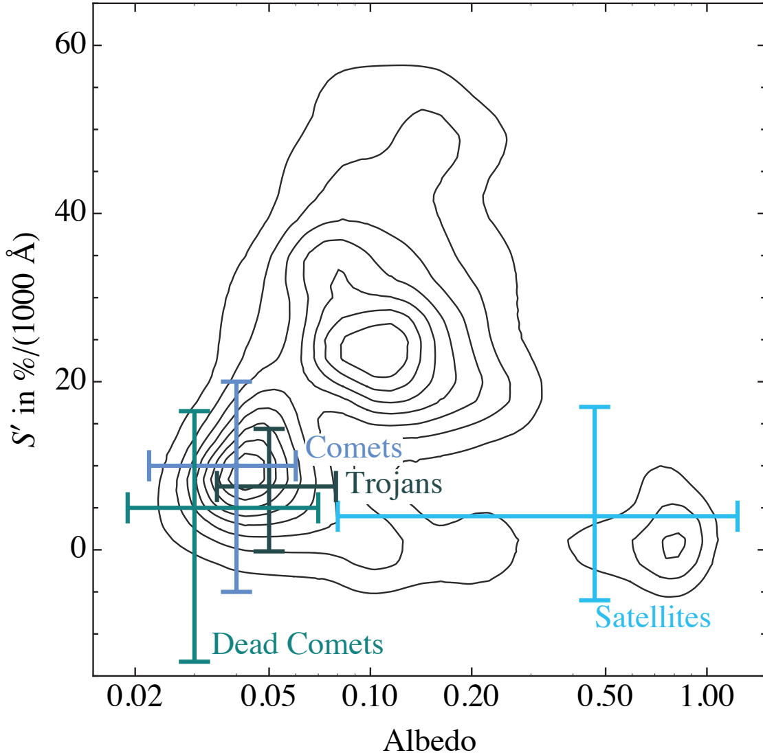
Fig. 4.— Albedo and color ranges (central 95%) for small body populations in the inner/intermediate solar system superimposed on TNO data contours (Figure 3). Comet data include Jupiter family and Oort cloud comets. Jovian L4 and L5 Trojans are included, and satellites of the giant planets.
