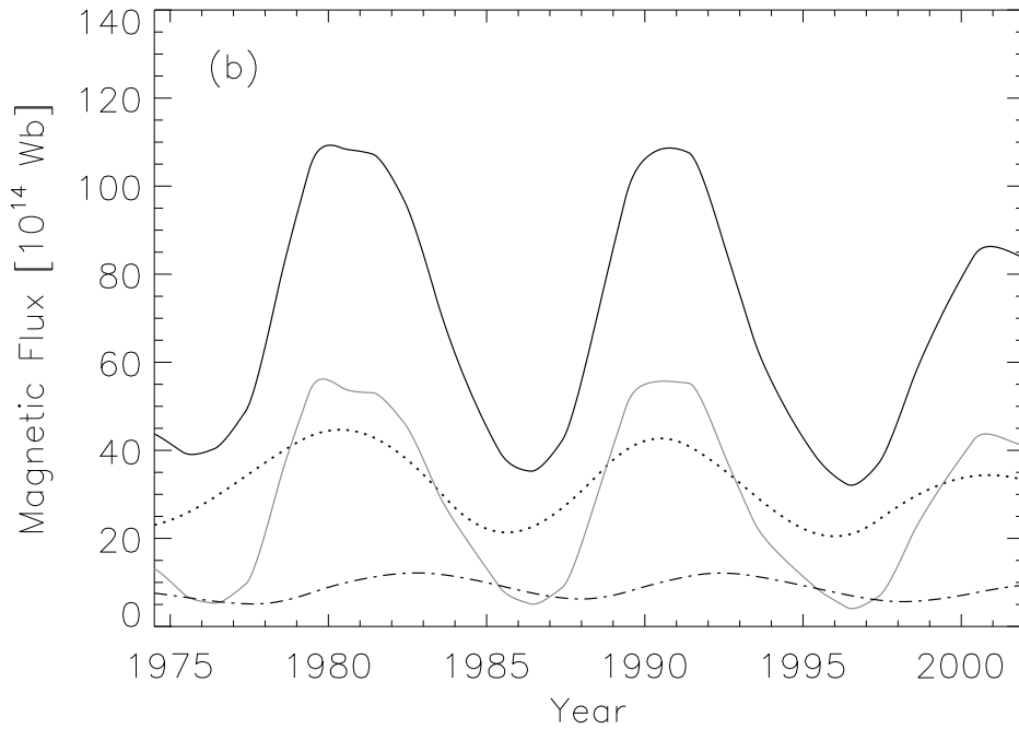
Fig. 1. (a): Total magnetic flux for individual Carrington rotations between 1974 and 2002. Different symbols represent data from synoptic charts obtained by different observatories (Arge et al., 2002). The solid line shows the magnetic flux calculated from the Group sunspot number. (b): Reconstructed magnetic flux in active regions (grey line), ephemeral regions (dotted), as well as the open (dot-dashed) and total flux (black line).
