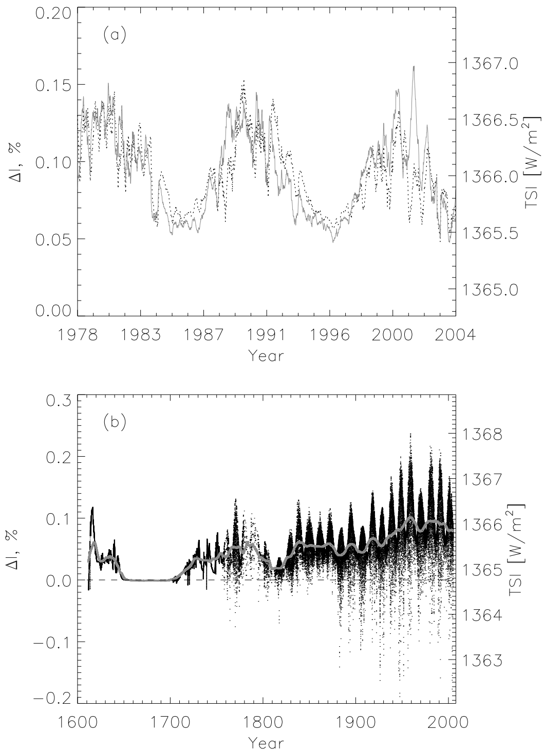
Fig. 3. (a): 3-month running mean of the daily sampled TSI for recent cycles: modelled (dots) and measured (solid line; PMOD composite). (b): Variation of the total solar irradiance since 1610. The grey solid line represents the 11-yr running mean of this variation.
