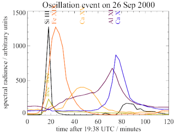
Figure 4. Multi-temperature light curves. During the initial phase emission is seen in all temperatures, peak temperatures are reached within minutes. The cooling lasts over 1 hour and comes to a sudden end. During the cooling the plasma is isothermal, i.e. at one temperature at a given time.
