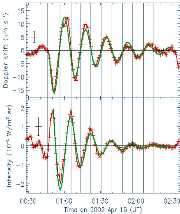
Figure 2. Doppler shift and spectral radiance (background trend removed) of the Fe XIX emission during a DOE. After a sudden start, the loops oscillate about a zero position corresponding to the rest wavelength. The phase shift is exactly 90^\circ (Wang 2003b). This is a strong argument in favour of an axial slow mode standing wave.
