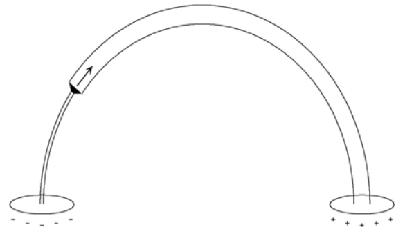
Figure 6. Cartoon of the empirical pinch model. The presented model can explain all observed features, in particular the rule of unidirectionality. It requires a potential difference between the foot points and a dominant polarity of the trigger area. This is also true for the magnetic polarity of the active foot point. More observations are needed to refine and test the presented model.
