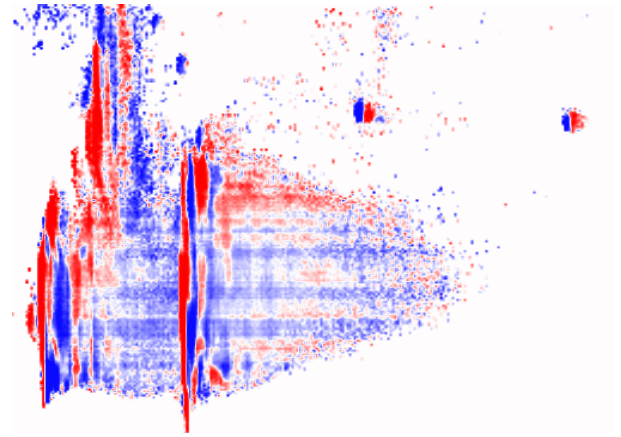
Figure 3. Doppler map of two double events. The loop, which has been hit by a DOE is unchanged and still in place, when another homologous trigger occurs. It seems to be a common feature that multiple events always start in the same direction, which implies that it is always the same foot point that generates the trigger.
