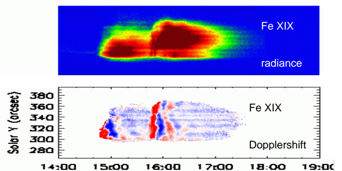
Figure 1. A recurring event observed in Fe XIX 1118 Å (6.7 MK). DOEs have a signature on both spectral radiance (top) and Doppler flow (bottom). The oscillatory nature is best seen in the velocity map v(x,t) .
