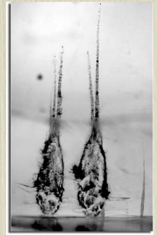
Tracks in Aerogel
